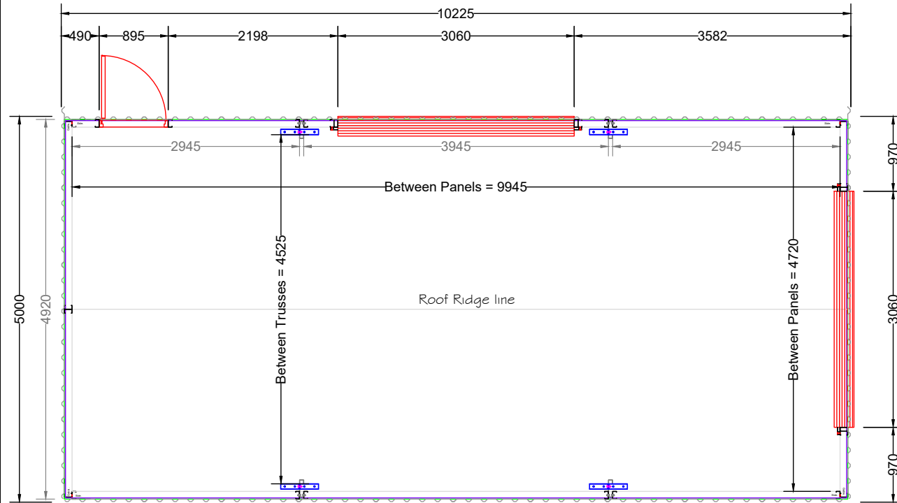
Plan View 1:50
